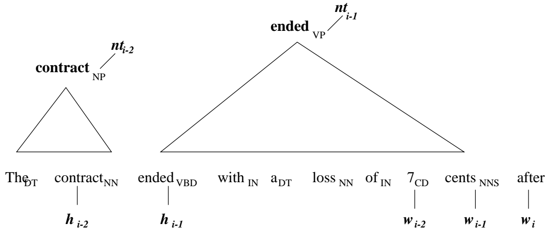
Figure 1: An Example of a Partial Parse (reproduced from Chelba & Jelinek (1998)).
